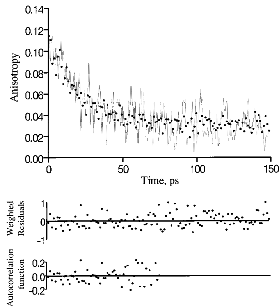
Figure 5. Examples of simulation-based fit (●) of the tetramer fluorescence anisotropy decay (—); \lambda_{\text{exc}} = 465 nm, \lambda_{\text{det}} = 612 nm; D_{||} = D_{\perp} = 0 .
